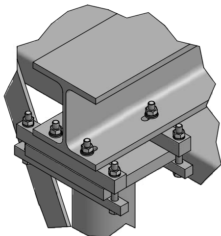
A: ATTACCO PIASTRA PISTONE PISTON PLATE FIXING
